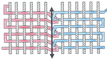
STRAIGHT INTERLOCK - COMMON WEFT
