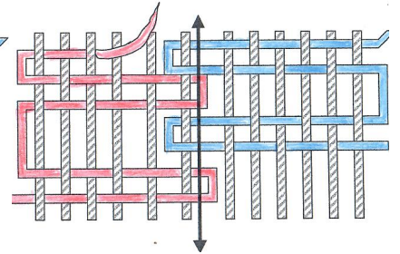
DIAGONAL INTERLOCK - COMMON WARP
